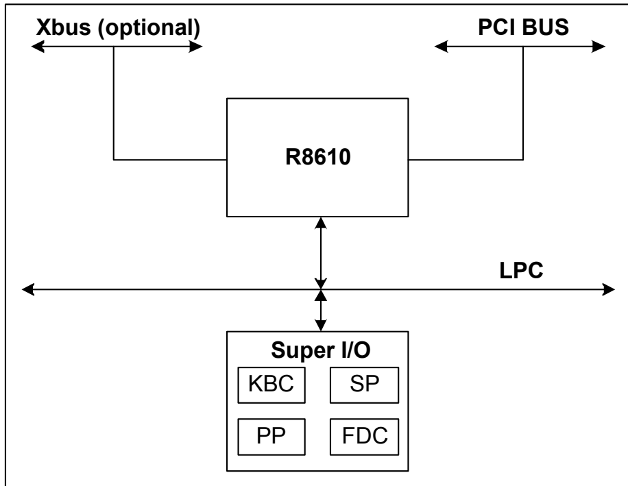
Figure 10-5. Typical Setup
