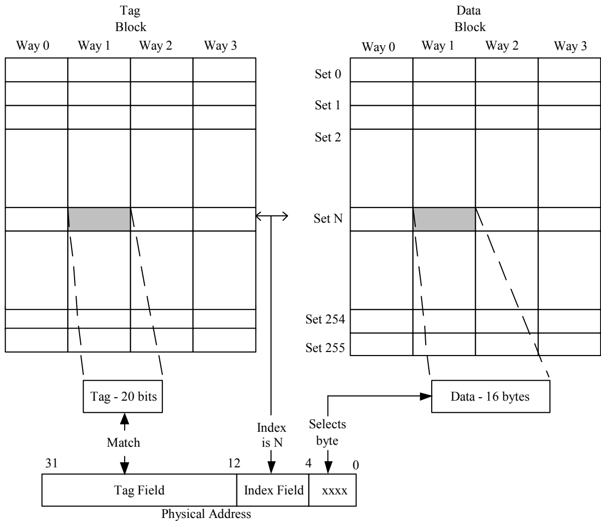
Figure 10-6. R8610 L1 Cache Architecture
