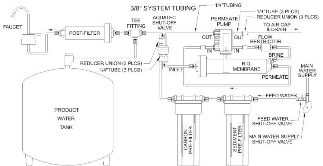
Figure 4. Typical R.O. System after installation of Permeate Pump with Aquatec shut-off valve that uses 1/4" JG connections – Part# PASV2000
