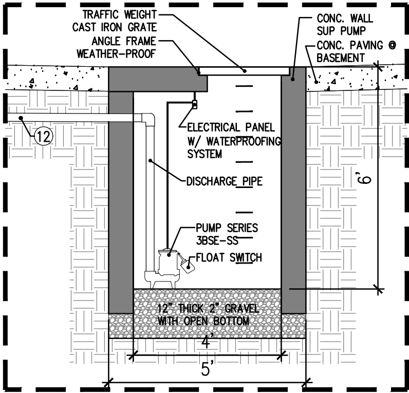
PUMP STATION DETAIL SCALE: NTS
