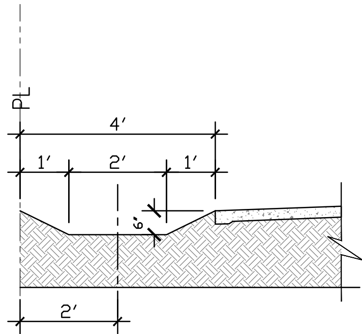
BIO-SWALE DETAIL SCALE: 1/2" = 1'-0"
